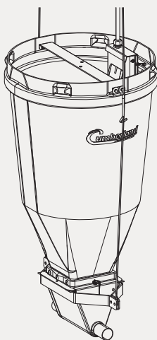
HOPPER FEED LEVEL CONTROL
