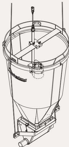
IR HOPPER SENSOR/CONTROL
